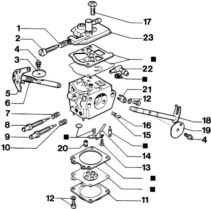
25 CARBURATORE COMPLETO COMPLETE CARBURETOR
